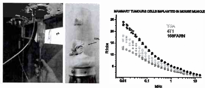
Fig 1. A) Photographs of the "in vivo" 11mm solenoid detection coil of FFC-NMR; B) "In vivo" 1/T_1 NMRD profiles of tumours obtained from transplantation of three mammary adenocarcinoma cell lines.
